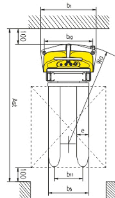
CDD10B - III / CDD15B - III Overall forks
